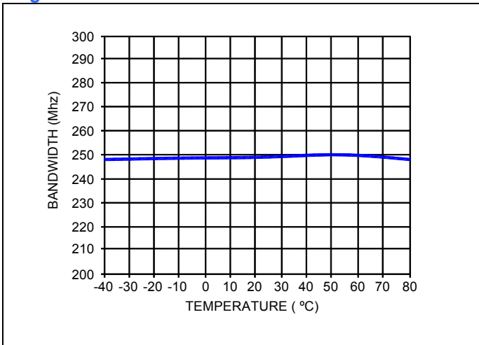
Fig. 3 : AMPLIFIER BANDWIDTH vs TEMPERATURE
